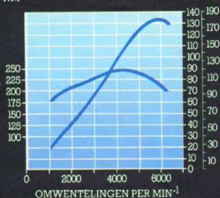
Prestatie/omwenteling-kurve 3.0 E
