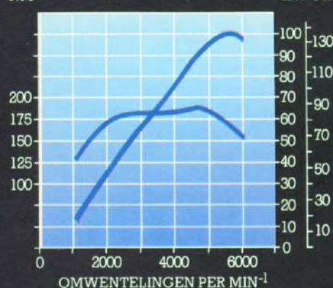
Prestatie/omwenteling-kurve 2.5 E
